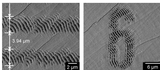
Figure 2. Scanning electron micrographs of the \text{CaCO}_3 crystals formed on the photoimaged PVA–SbQ matrix in the presence of PAA.
